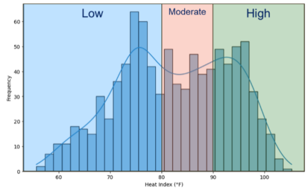
Figure 10 Heat Index Distribution for Historical Weather Data During Summer Months from 2015 to 2024 in Tokyo
